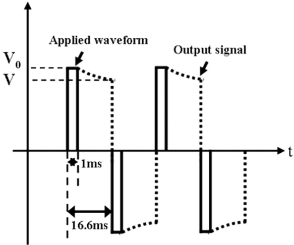
FIGURE 6 Schematic applying a 60 Hz square waveform and output signal of the measurement.
