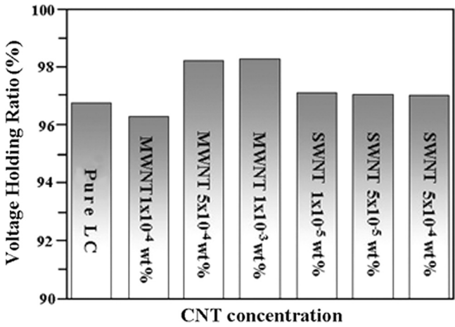
FIGURE 7 Measured voltage holding ratio characteristics according to CNT concentration.
